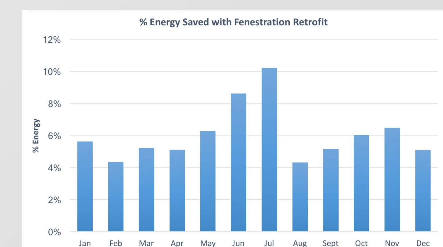
The percentage of energy saved in Gilbert-Addoms each month by the fenestration retrofit if maximum energy savings were achieved.
